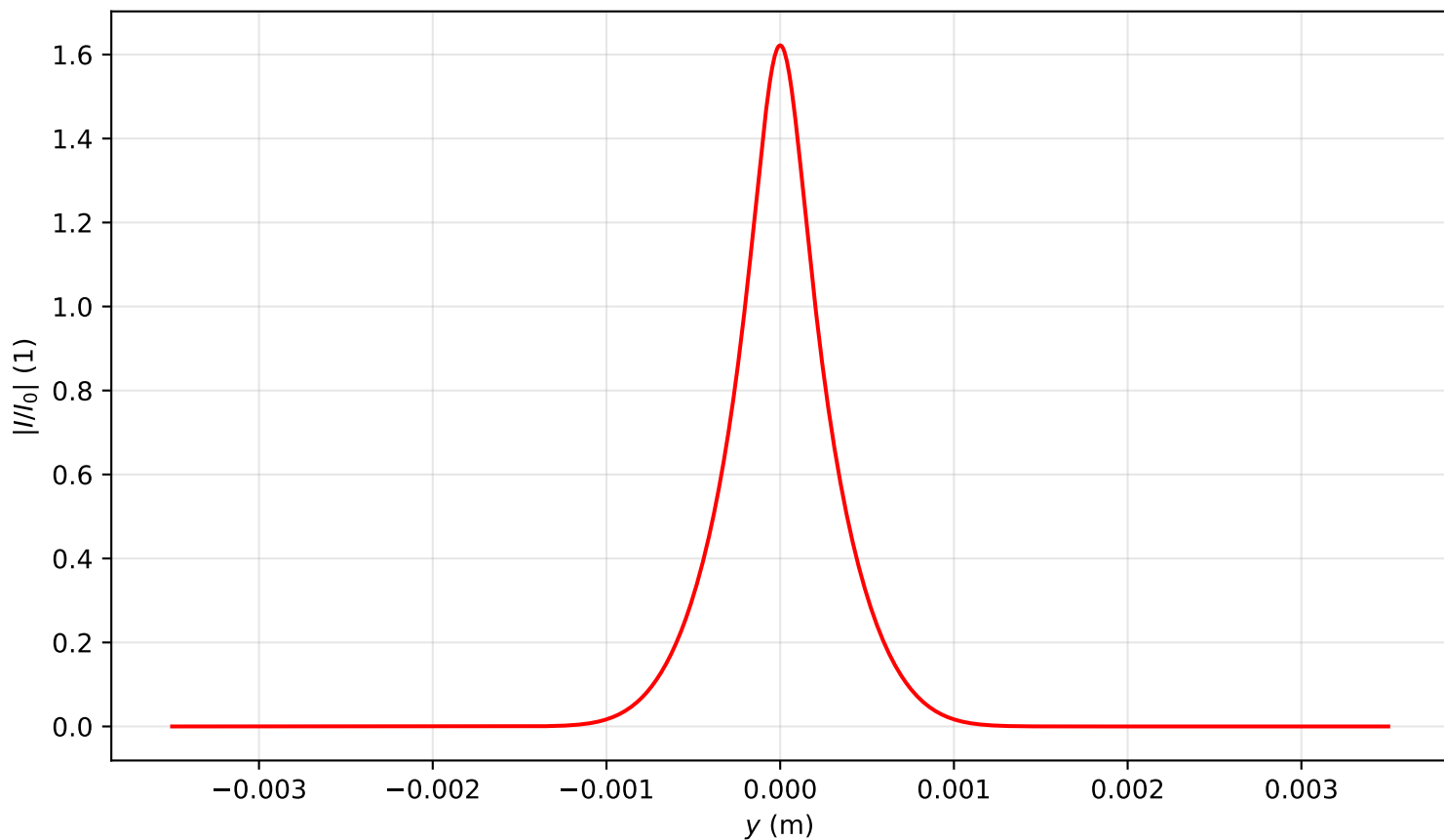
Intensity profile I(x=0, y, z=0.239)/I_0 , \text{Pin}=6.5\text{Pcr} , artificial time
